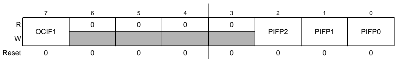
Figure 2-24. Port P Interrupt Flag Register
