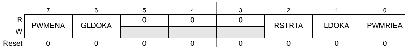
Figure 14-24. PMF Enable Control A Register (PMFENCA)
