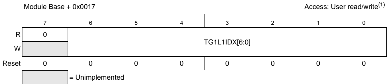
Figure 13-20. Trigger Generator 1 List 1 Index (TG1L1IDX)
