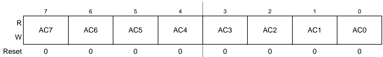
Figure 12-20. MSCAN Identifier Acceptance Registers (First Bank) — CANIDAR0–CANIDAR3
