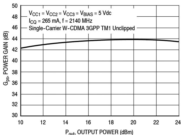
Figure 26. Power Gain versus Output Power
