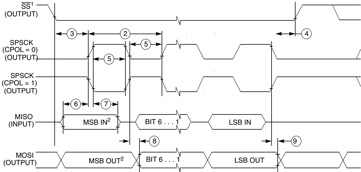
Figure 6. SPI master mode timing (CPHA=0)
