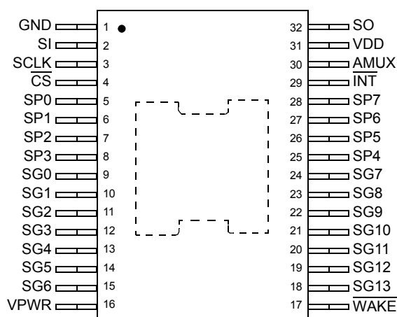
Figure 3. 34975 Pin Connections
