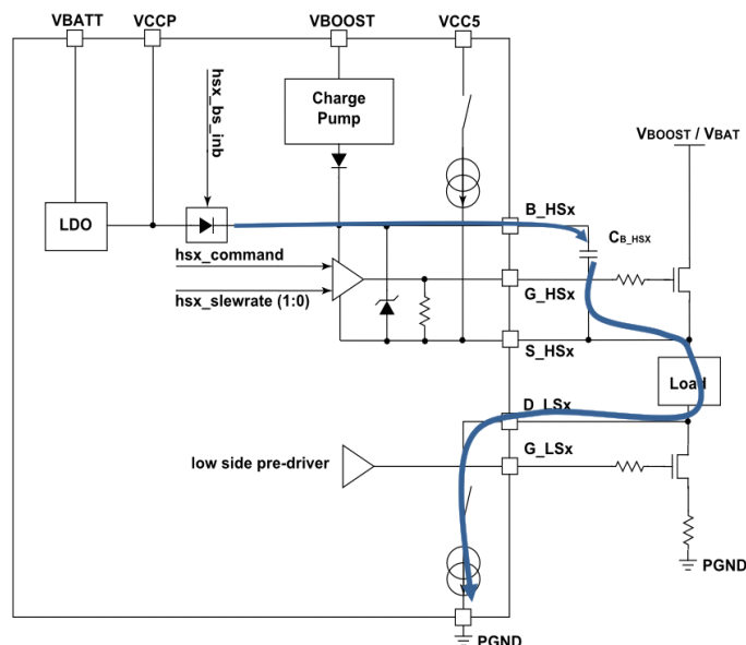
Figure 14. Booststrap Load Current Path During Start-up Default Sequence
