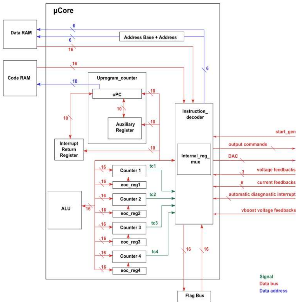
Figure 34. Microcore Block Diagram
