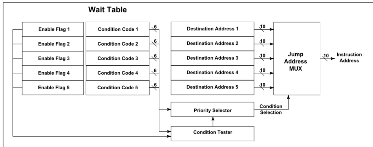
Figure 43. Wait Table Management Diagram
