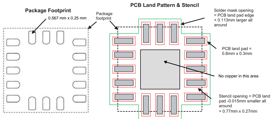
Figure 18. Recommended PCB land pattern, solder mask, and stencil opening near package footprint
