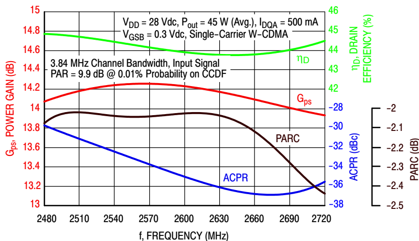
Figure 3. Single-Carrier Output Peak-to-Average Ratio Compression (PARC) Broadband Performance @ P_{out} = 45 \text{ Watts Avg.}
