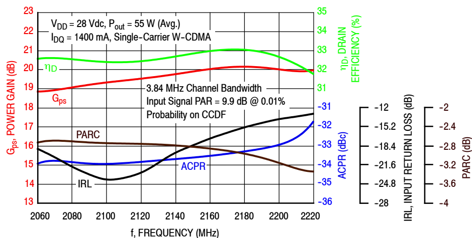
Figure 4. Single-Carrier Output Peak-to-Average Ratio Compression (PARC) Broadband Performance @ P_{out} = 55 \text{ Watts Avg.}
