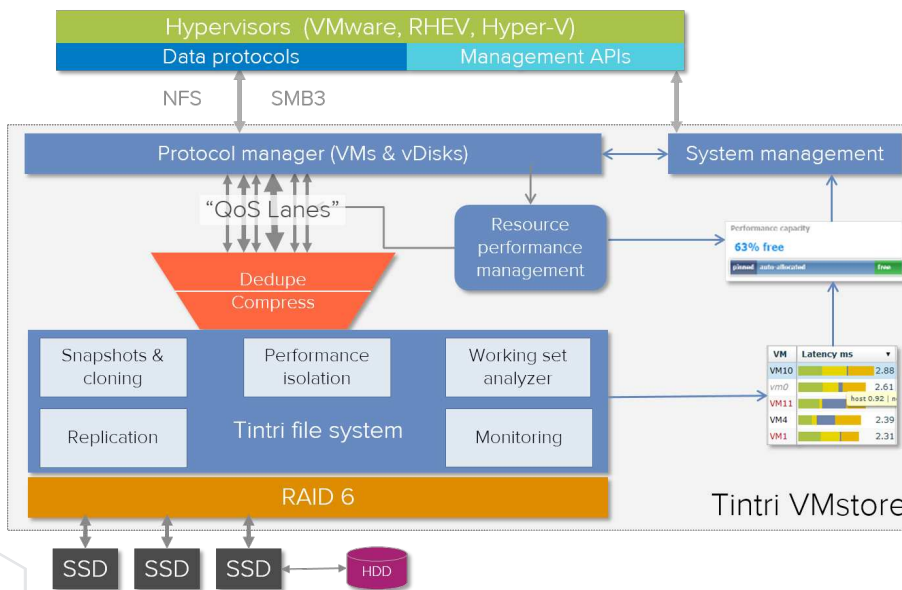
Figure 1: Architectural diagram of Tintri Operating System.
