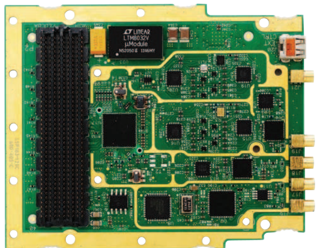
Radio420S FMC
