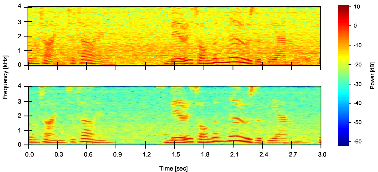
Speech signal and its energy distribution over frequency and time: Input signal and ANC result
