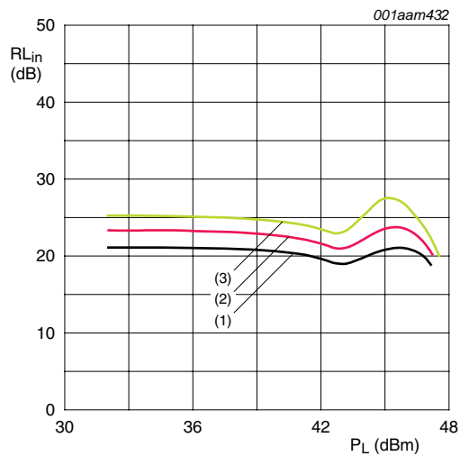
V_{DS} = 28\text{ V} ; I_{DQ} = 170\text{ mA} ; V_{GS(amp)peak} = 0\text{ V} ; T_{case} = 25\text{ }^\circ\text{C} ; \delta = 10\% ; t_p = 100\text{ }\mu\text{s} on 1 ms period. (1) f = 2010\text{ MHz} (2) f = 2018\text{ MHz} (3) f = 2025\text{ MHz}
