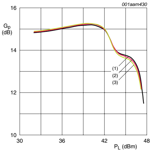
V_{DS} = 28\text{ V} ; I_{DQ} = 170\text{ mA} (main); T_{case} = 25\text{ }^\circ\text{C} ; V_{GS(amp)peak} = 0\text{ V} ; \delta = 10\% ; t_p = 100\text{ }\mu\text{s} on 1 ms period. (1) f = 2010\text{ MHz} (2) f = 2018\text{ MHz} (3) f = 2025\text{ MHz}
