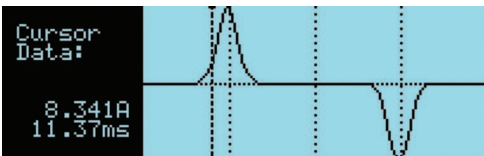
Acquired Current waveform (MX30/45 Display).
