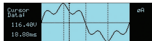
Acquired Voltage waveform (iX Display).
