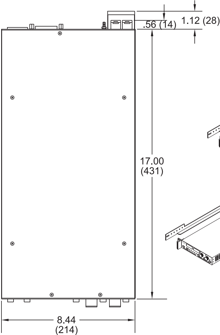
Top View
