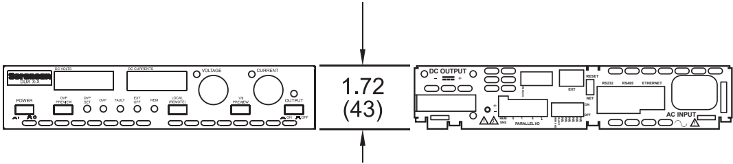
Front View
