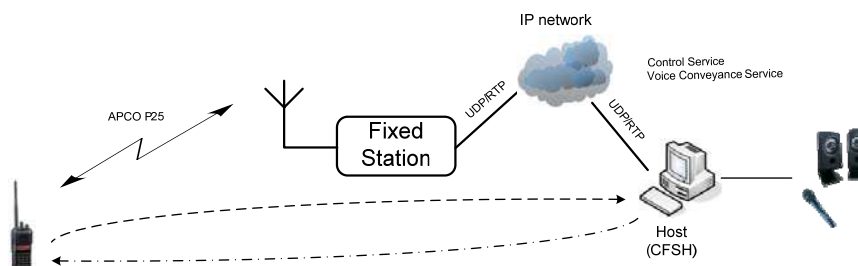
Figure: Digital Fixed Station Interface
