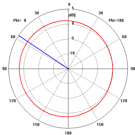
Image 4: polar radiation pattern, yz plane
