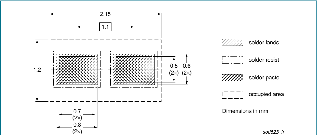
Fig 15. Reflow soldering footprint PESD5V0V1BB (SOD523/SC-79)
