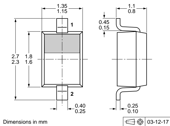
Fig 7. Package outline PESD5V0L1UA (SOD323/SC-76)
