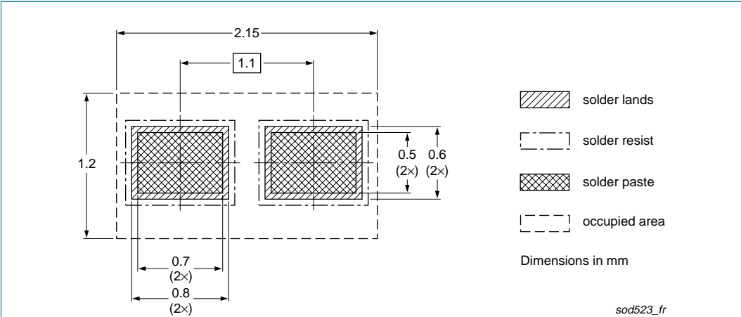
Fig 12. Reflow soldering footprint PESD5V0L1UB (SOD523/SC-79)
