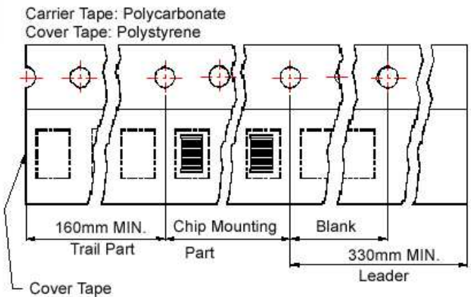
Tape Material
