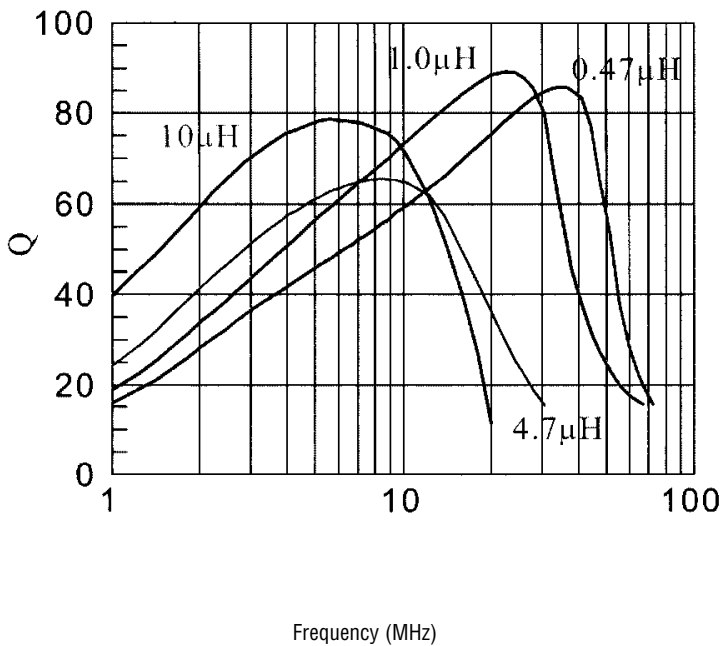
TEST EQUIPMENT: HP4284, HP-4291 Q-VALUE CURVES
