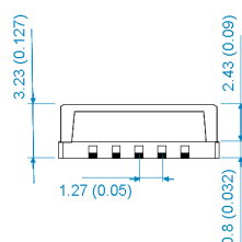
MS9000 side view
