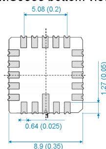
MS9000 bottom view
