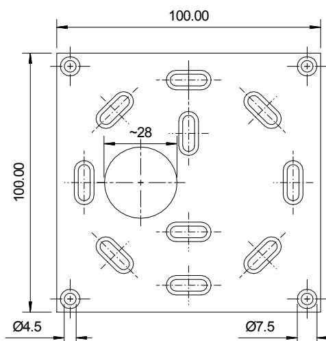
Mounting bracket
