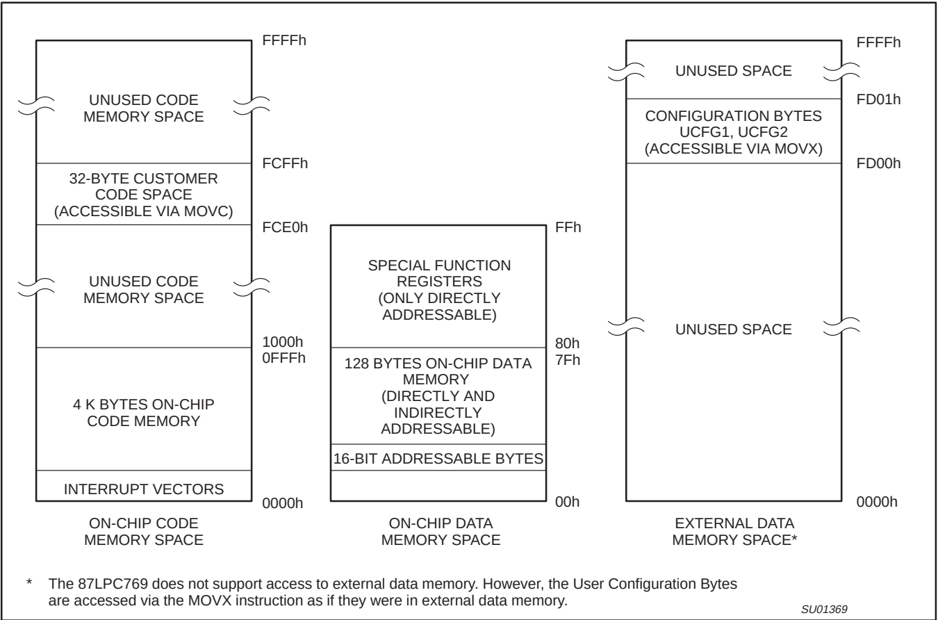
Figure 1. P87LPC769 Program and Data Memory Map
