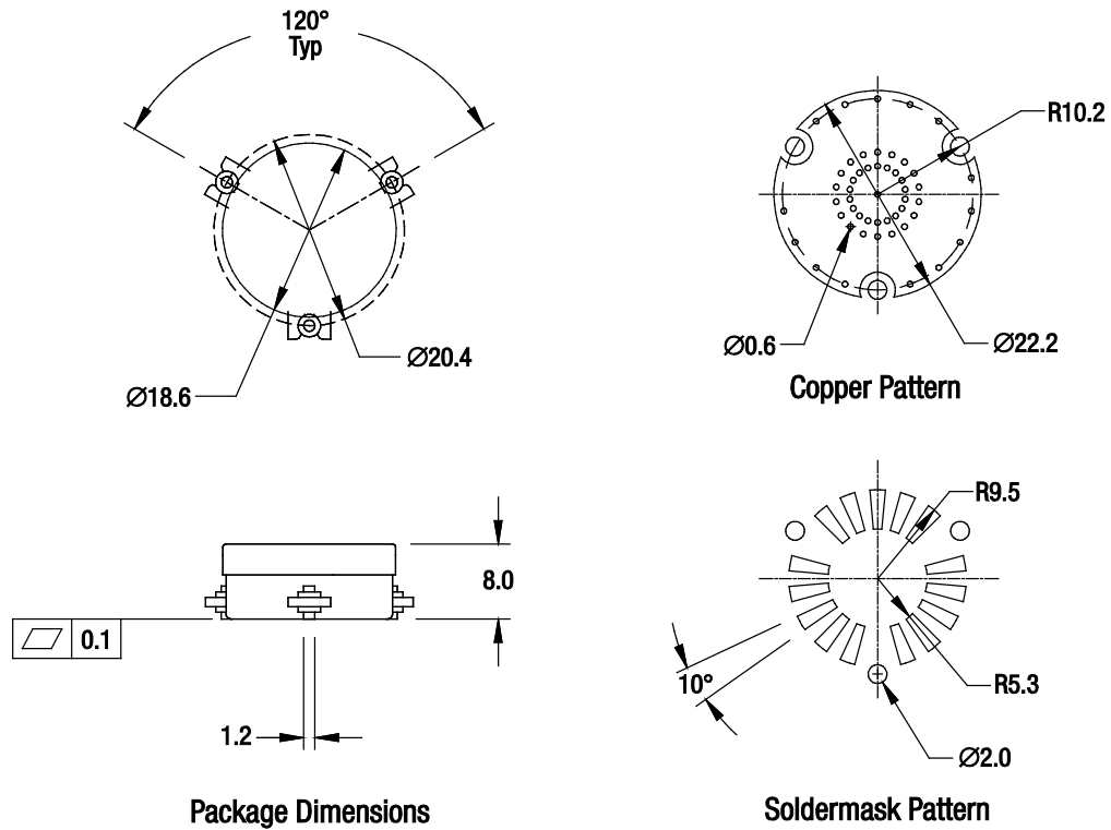
Figure 2. MAFR-000653-000001 Package Dimensions
