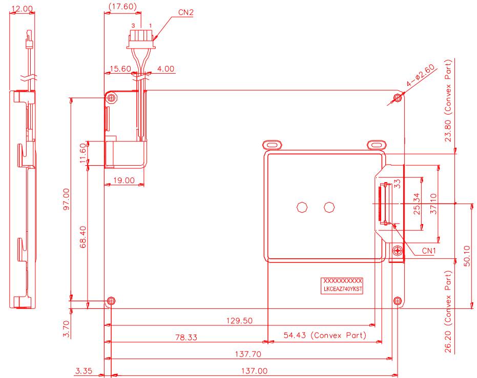
INTERFACE FOR CN2:JST BHR-03VS-1
