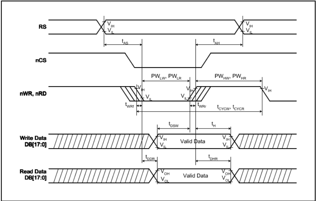
Figure 50 i80-System Bus Timing
