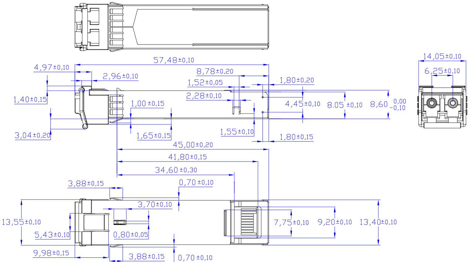
Figure 5, Mechanical Design Diagram of the SFP
