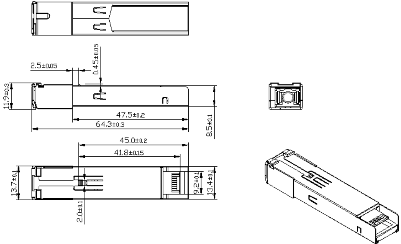
Figure 4 Mechanical Diagram
