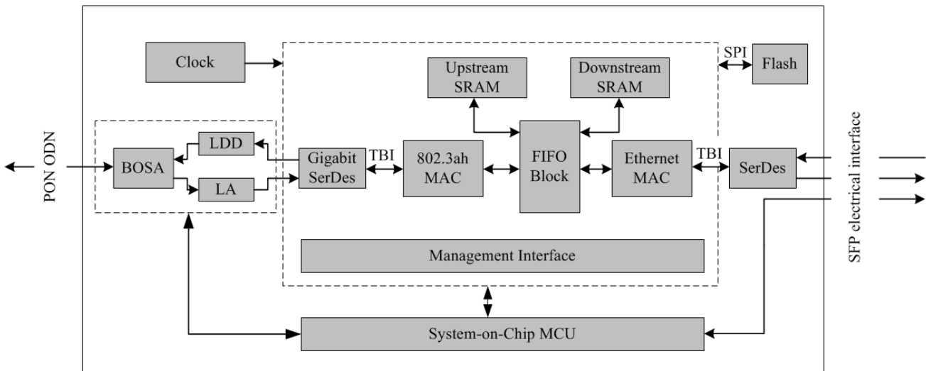
Figure 1, SPS-34-GB-P2-EDFN Block Diagram
