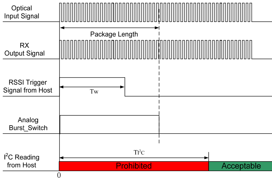
Figure 7, RSSI Timing Diagram
