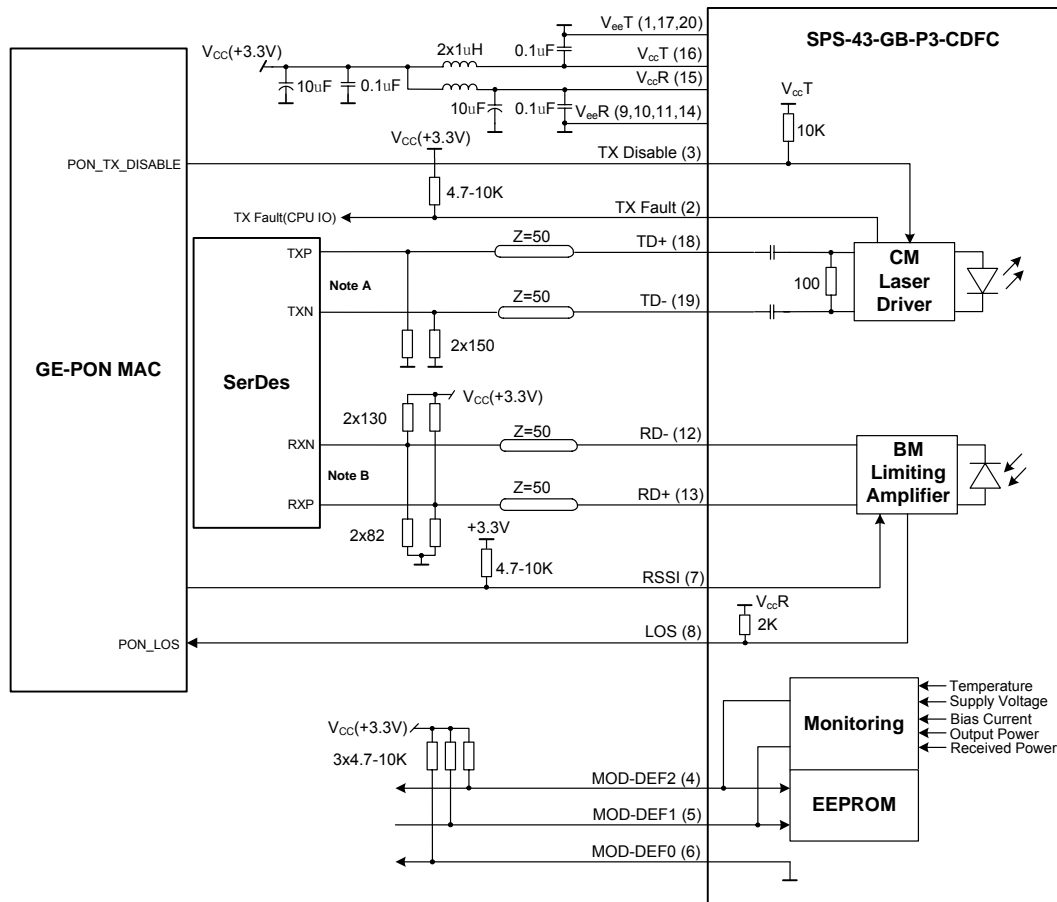
Figure 5, Recommended Interface Circuit
