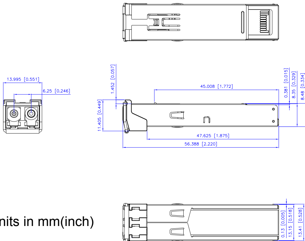
Figure 9 Mechanical Diagram
