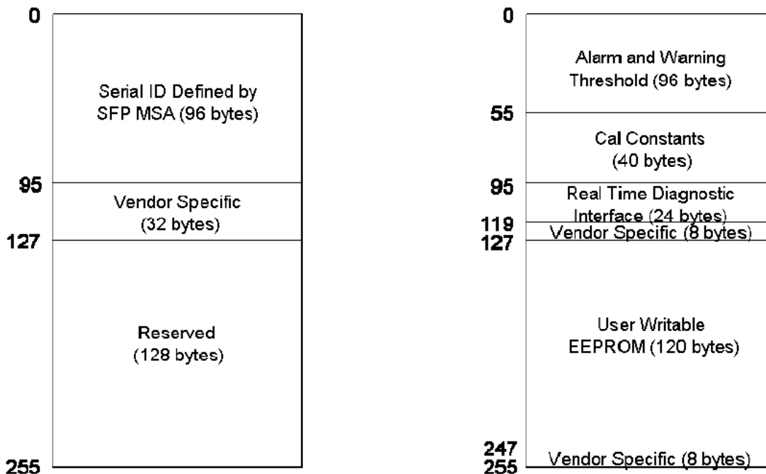
Figure 8, 2-wire Serial Digital Diagnostic Memory Map
