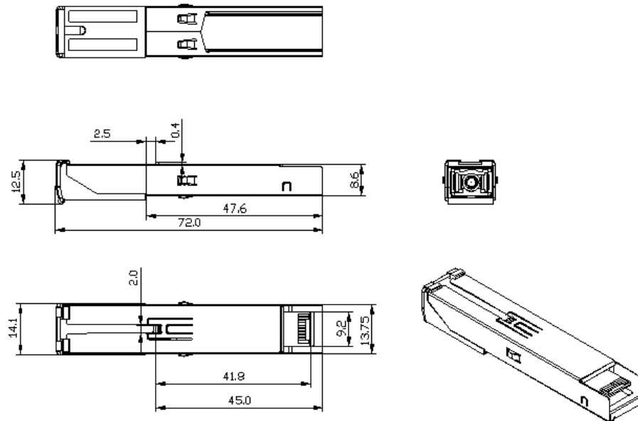
Figure 3, Mechanical Diagram
