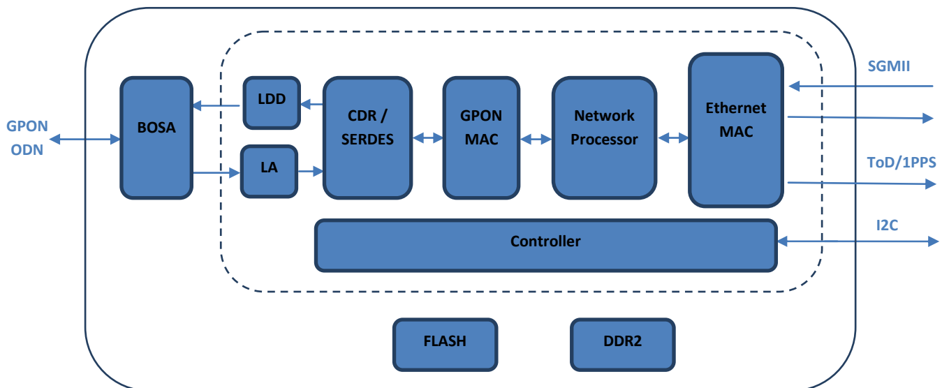
Figure 1, Block Diagram
