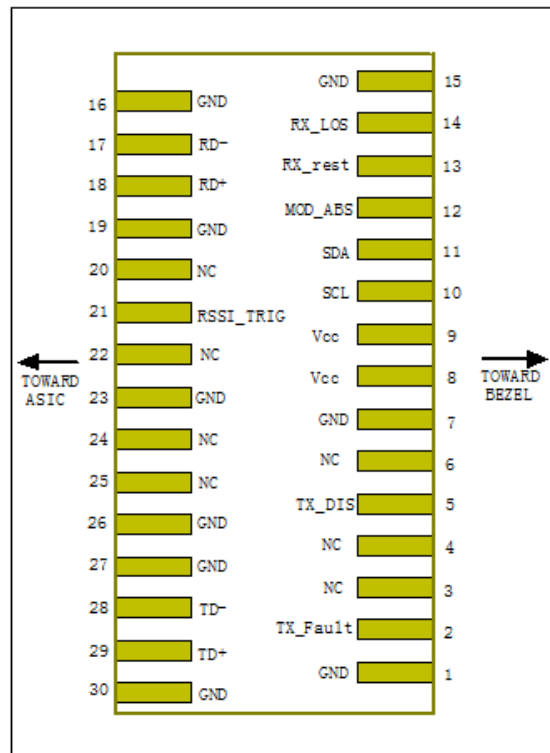
Figure5, XFP Pin View (Golden Finger)
