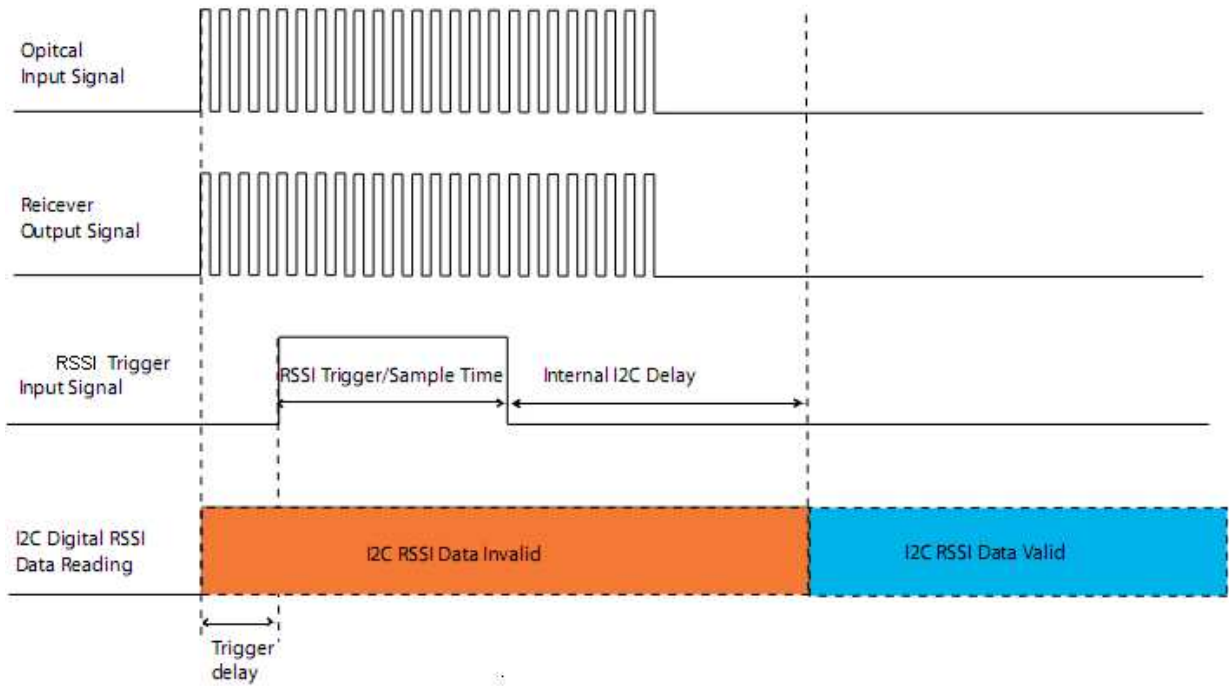
Figure 2, RSSI Timing Specification
