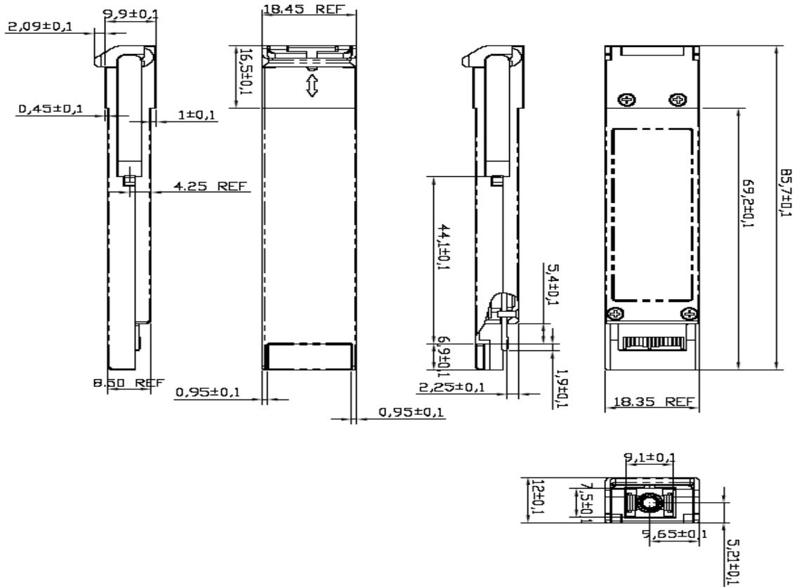
Figure 6, Mechanical Diagram
