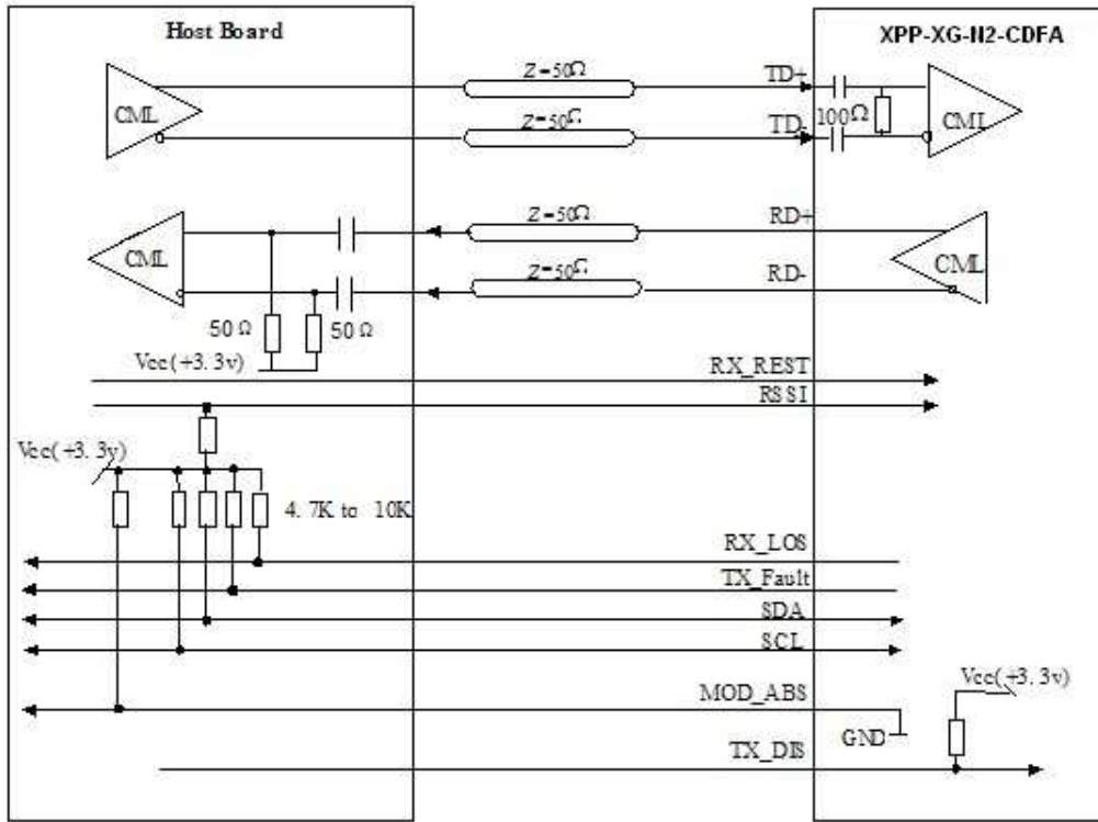
Figure 4, Recommended Interface Circuit
