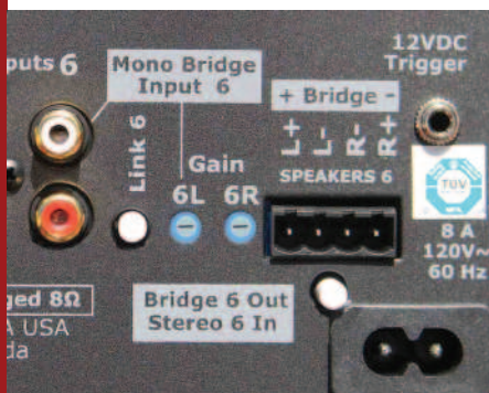
MX1255 rear panel shown
