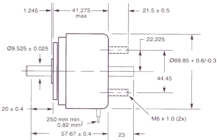
Solenoid shown in energised position
