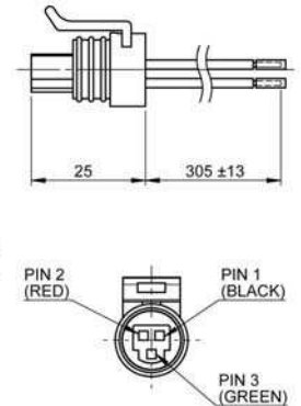
Mating Connector Packard Metri-Pack, Cable Assembly
