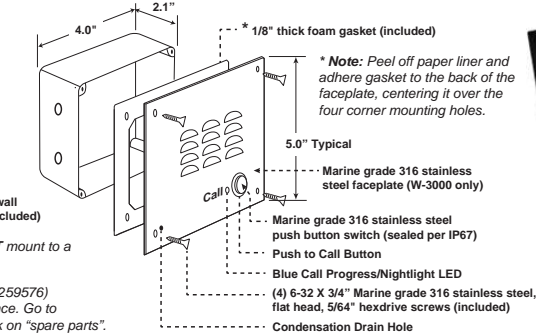
W-3000-EWP shown with optional Viking Model VE-5x5 Surface Mount Box and VE-GNP Gooseneck Pedestal
