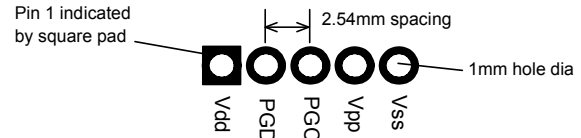
Figure 9. Recommended plate-through connector design
