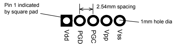
Figure 9. Recommended plate-through connector design
