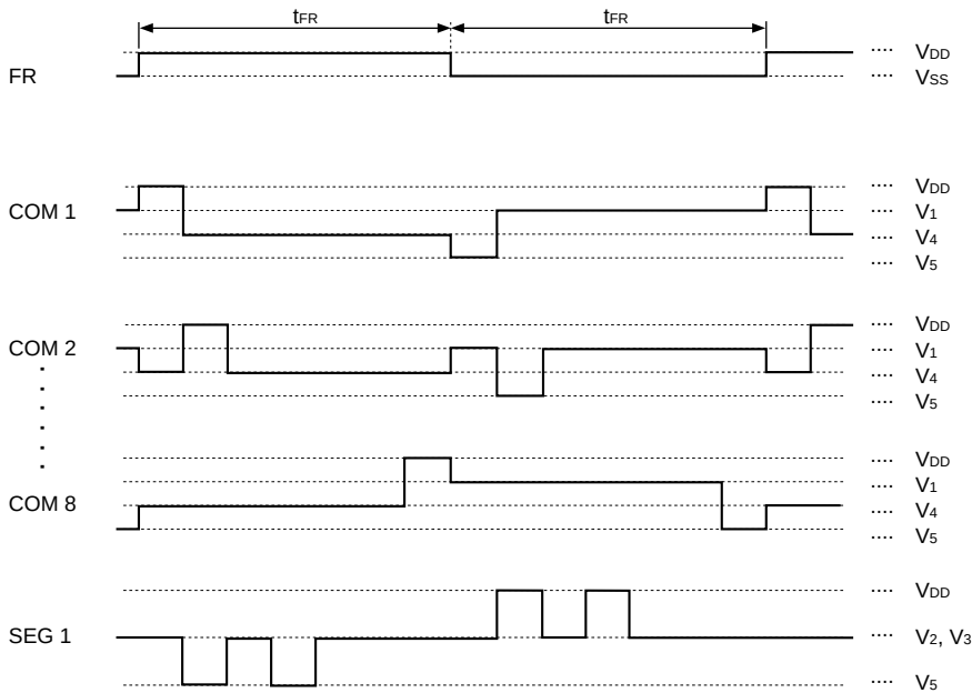
Figure 5 1/8 Duty Cycle Drive Waveforms
