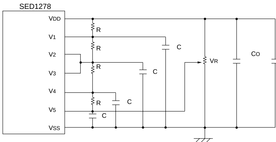
Figure 3 LCD Drive Voltage Network – 1/8 or 1/11 Duty Cycle
