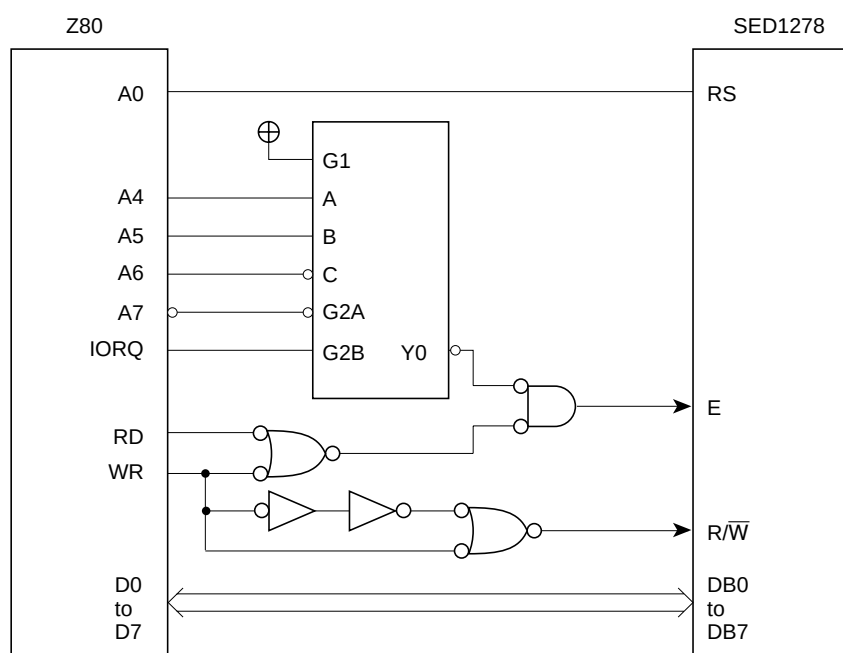
Figure 8 Interfacing the SED1278 to the Zilog Z80®
