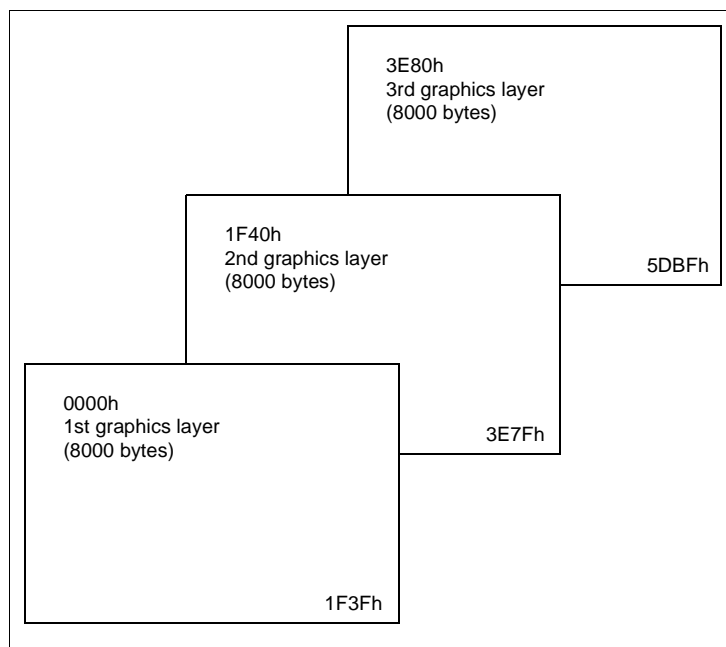
Figure 15-4 Three-Layer Graphics
