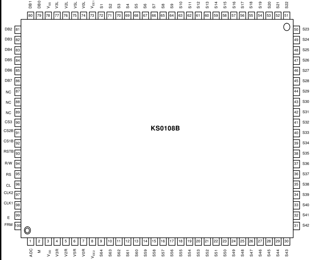
Fig.2. 100QFP Top View
