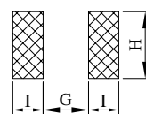
PCB PATTERN
