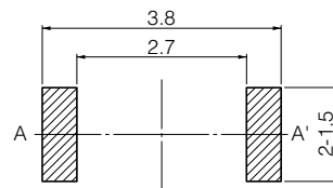
PWB land pattern for reference
