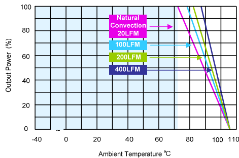
MTQZ50-72S12,MTQZ50-72S15,MTQZ50-110S15 Derating Curve without Heatsink
