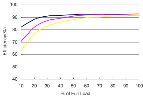
MKW140-48S24 Efficiency vs Load Current
