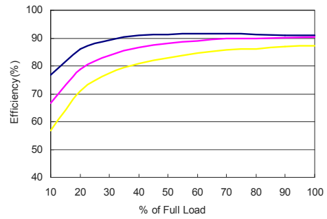
MKW140-48S05 Efficiency vs Load Current
