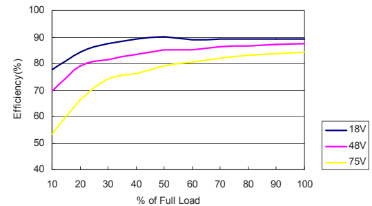
MKW140-48S15 Efficiency vs Load Current
