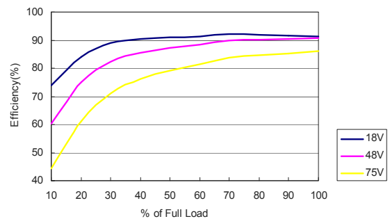
MKW140-48S05 Efficiency vs Load Current
