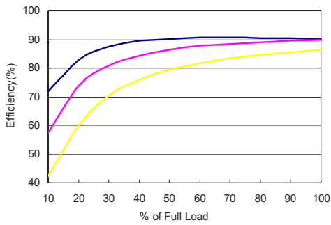
MKW140-48S033 Efficiency vs Load Current
