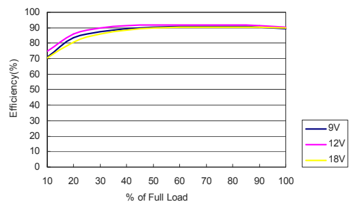
MKW40-12S05 Efficiency vs Load Current
