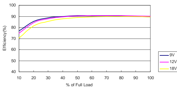
MJW25-12S12 Efficiency vs Load Current
