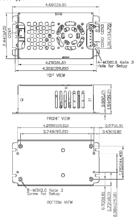
MEF Enclosed type
