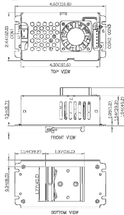
MDF -E Din rail type with FAN
