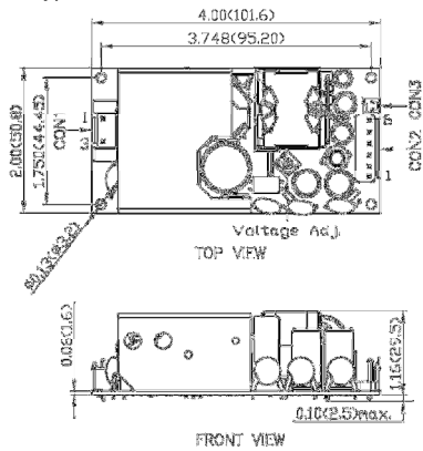
MAF Open type
