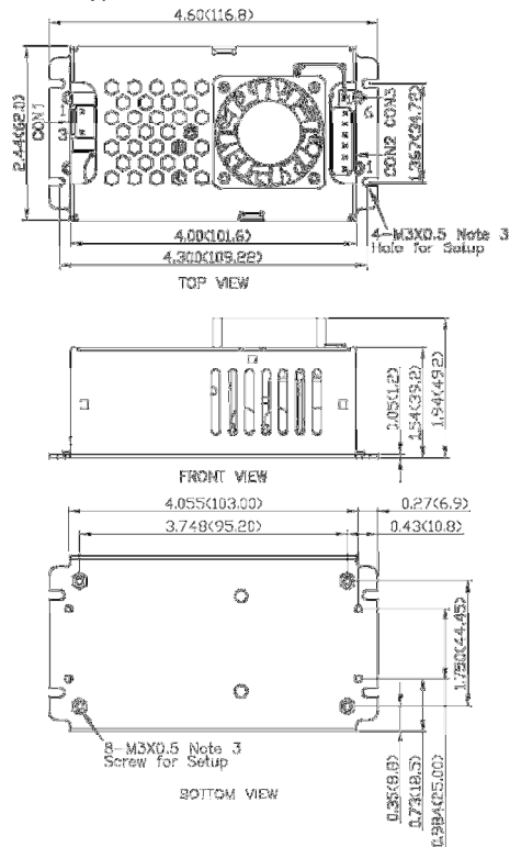
MEF -E Enclosed type with FAN
