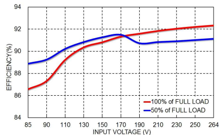
Efficiency vs. Input Voltage M□F150US24
