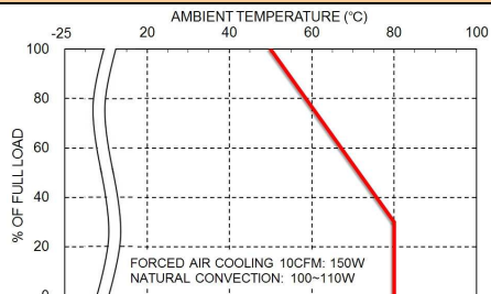
Derating Curve vs. Ambient Temperature M□F150
