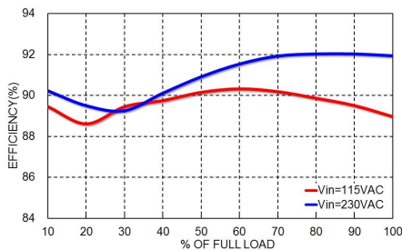
Efficiency vs. Output Load M□F150US24
