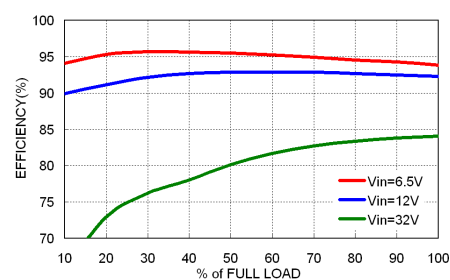
PSR1.0-05 Efficiency vs. Output Load
