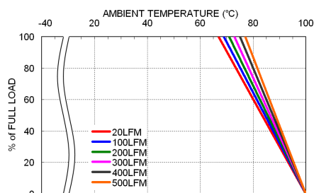
PSR1.0-05 Derating Curve
